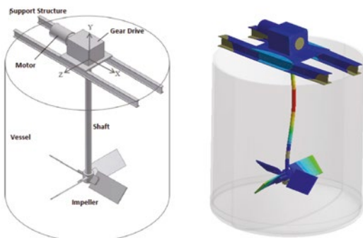
A modal analysis conducted on a typical large mixer-vessel structure system.
